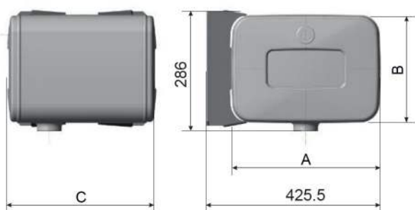
360 x 260 Profile
